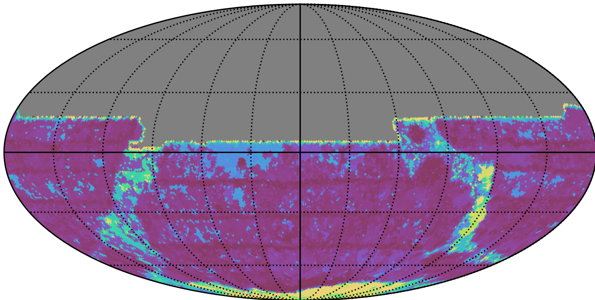
too_combined_s1.5_v3.4_10yrs All sky y band: Max Inter-Night Gap
