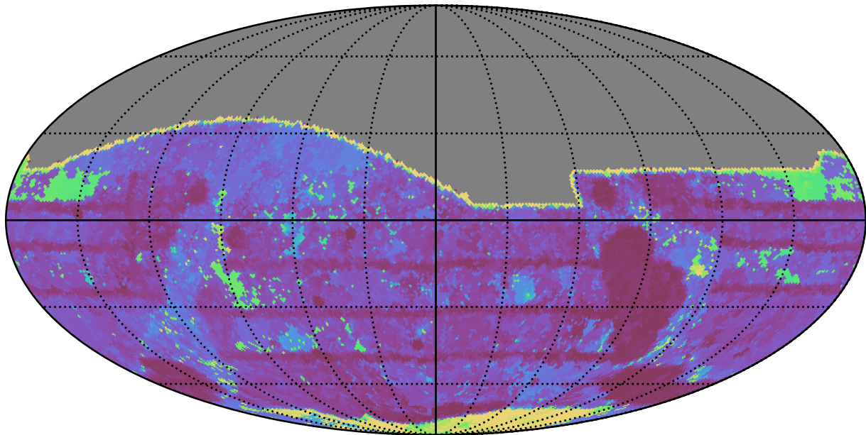
too_combined_s1.5_v3.4_10yrs All sky r band: Max Inter-Night Gap
