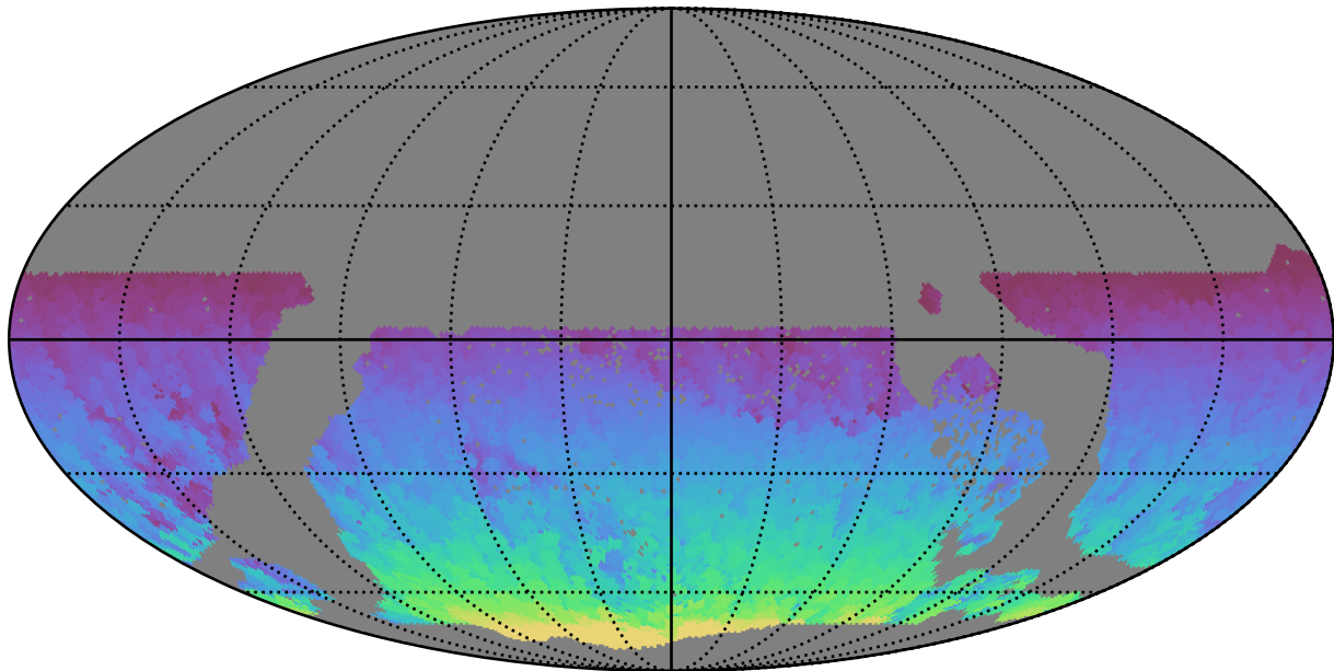
too_combined_s1.5_v3.4_10yrs WFD all bands: Max HA
