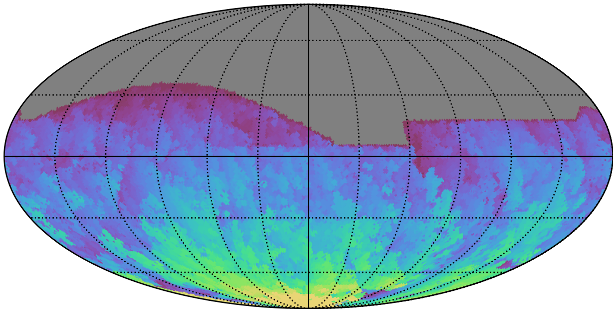
too_combined_s1.5_v3.4_10yrs All sky r band: Max HA
