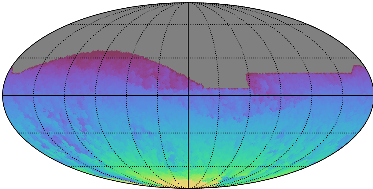
too_combined_s1.5_v3.4_10yrs All sky all bands: Max HA
