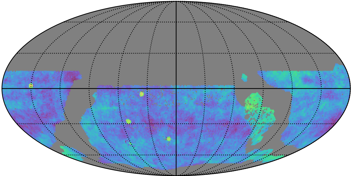
too_combined_s1.5_v3.4_10yrs gri WFD: Fraction of visits in pairs (20-90 min)
