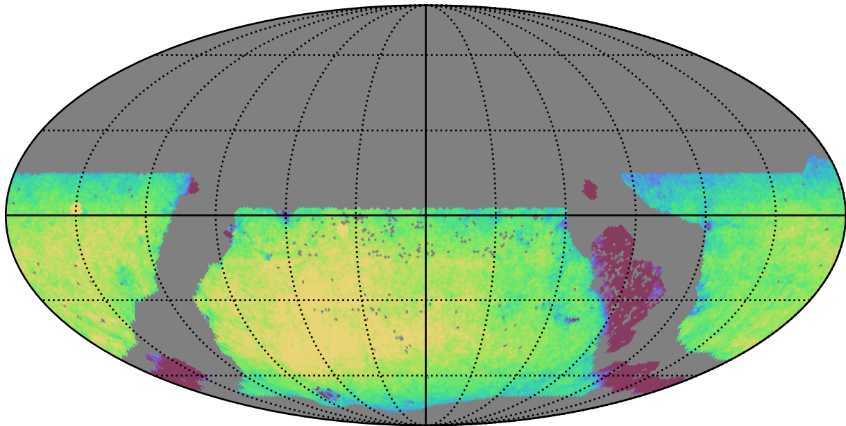
too_combined_s1.5_v3.4_10yrs WFD y band: Exgal_CoaddM5
