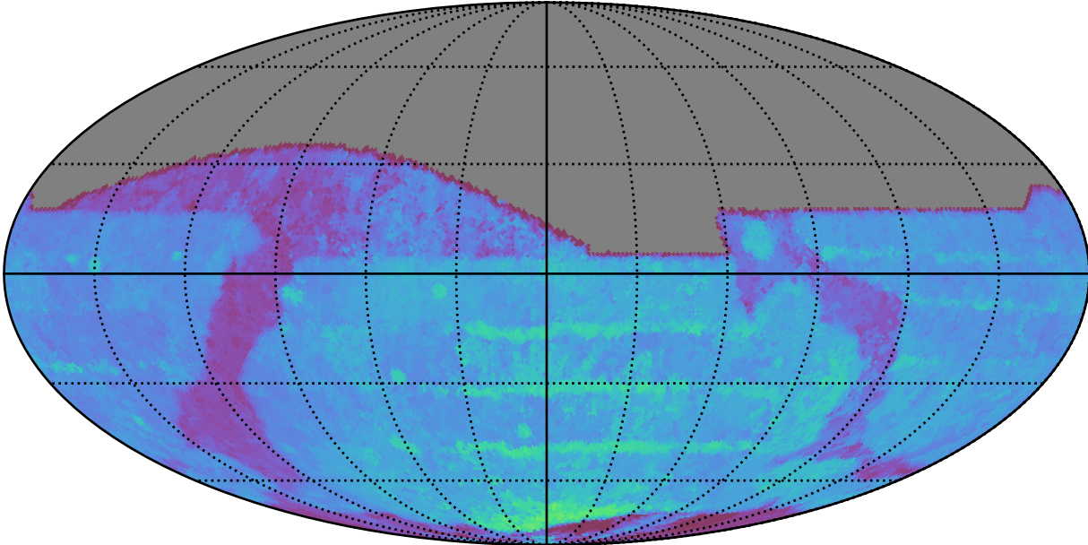
too_combined_s1.5_v3.4_10yrs All sky z band: 80thPercentile Season Length
