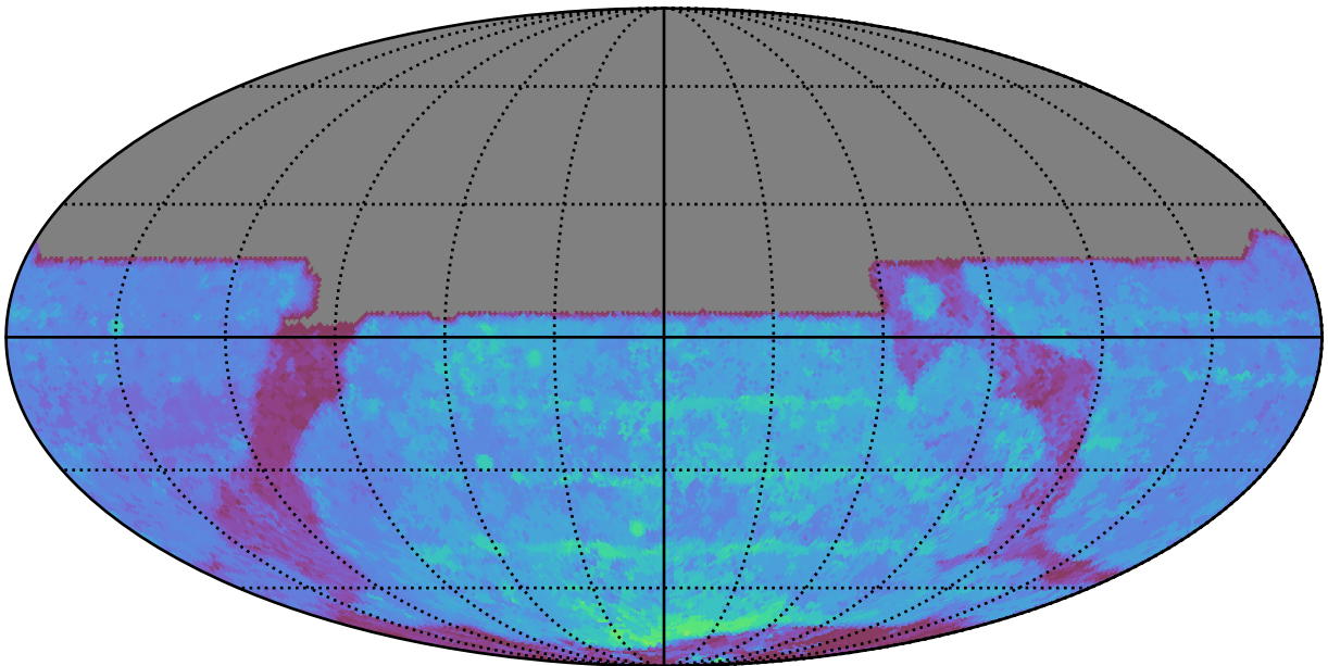
too_combined_s1.5_v3.4_10yrs All sky y band: 80thPercentile Season Length
