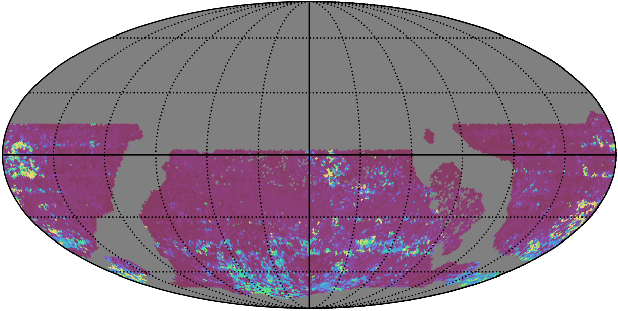
too_combined_s1.5_v3.4_10yrs WFD z band: 75th Percentile Intranight Timespan
