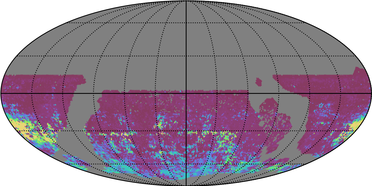
too_combined_s1.5_v3.4_10yrs WFD r band: 75th Percentile Intranight Timespan
