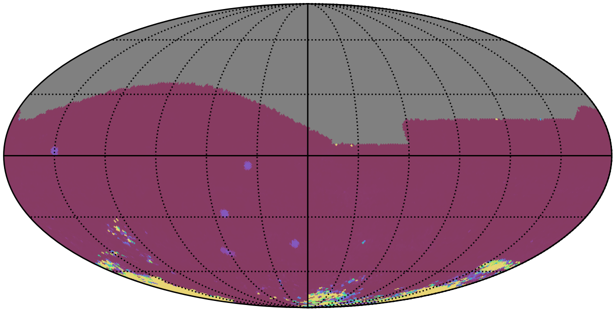
too_combined_s1.5_v3.4_10yrs All sky iz bands: 75th Percentile Intranight Timespan
