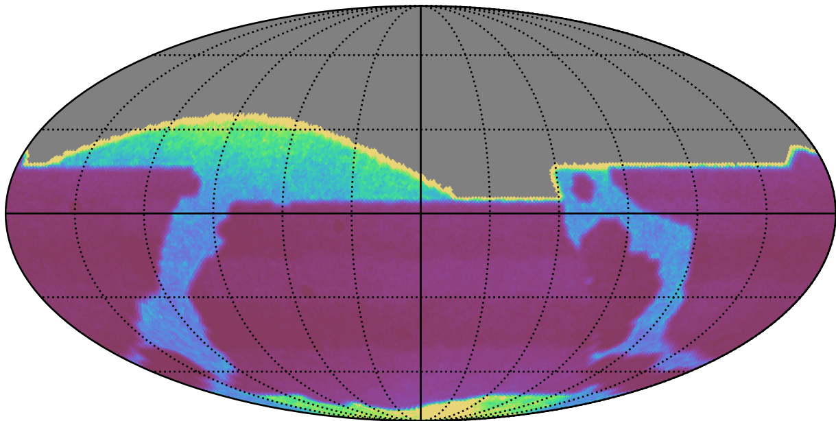
too_combined_s1.5_v3.4_10yrs : properMotion
