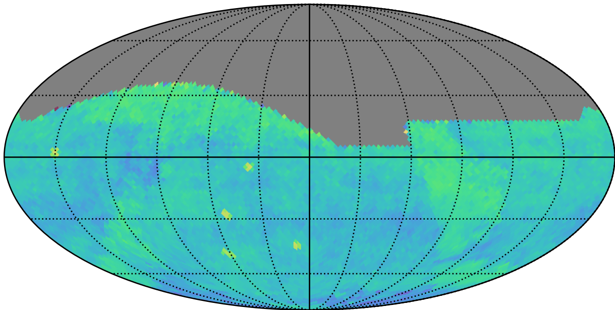
too_combined_s1.5_v3.4_10yrs (g or r or i): PairFraction
