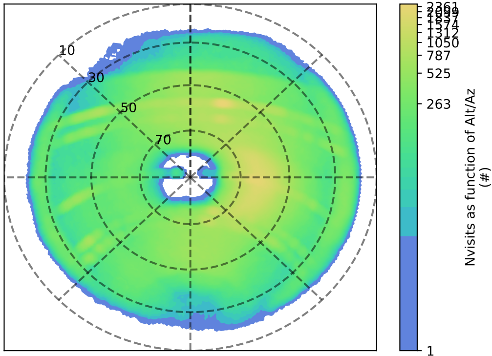
too_combined_s1.5_v3.4_10yrs z: Nvisits as function of Alt/Az
