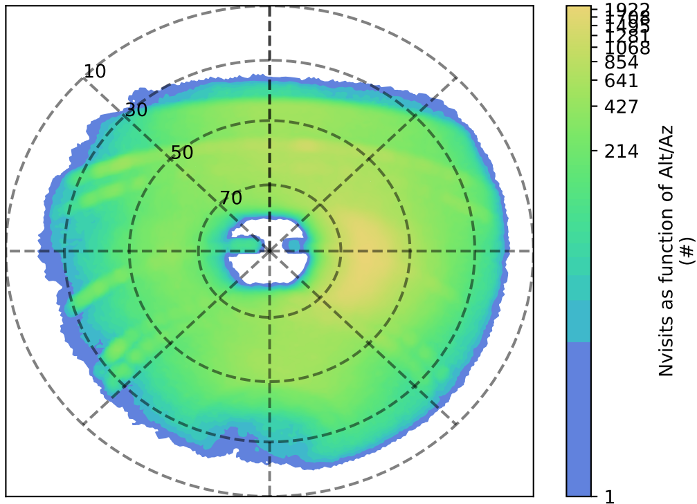
too_combined_s1.5_v3.4_10yrs y: Nvisits as function of Alt/Az
