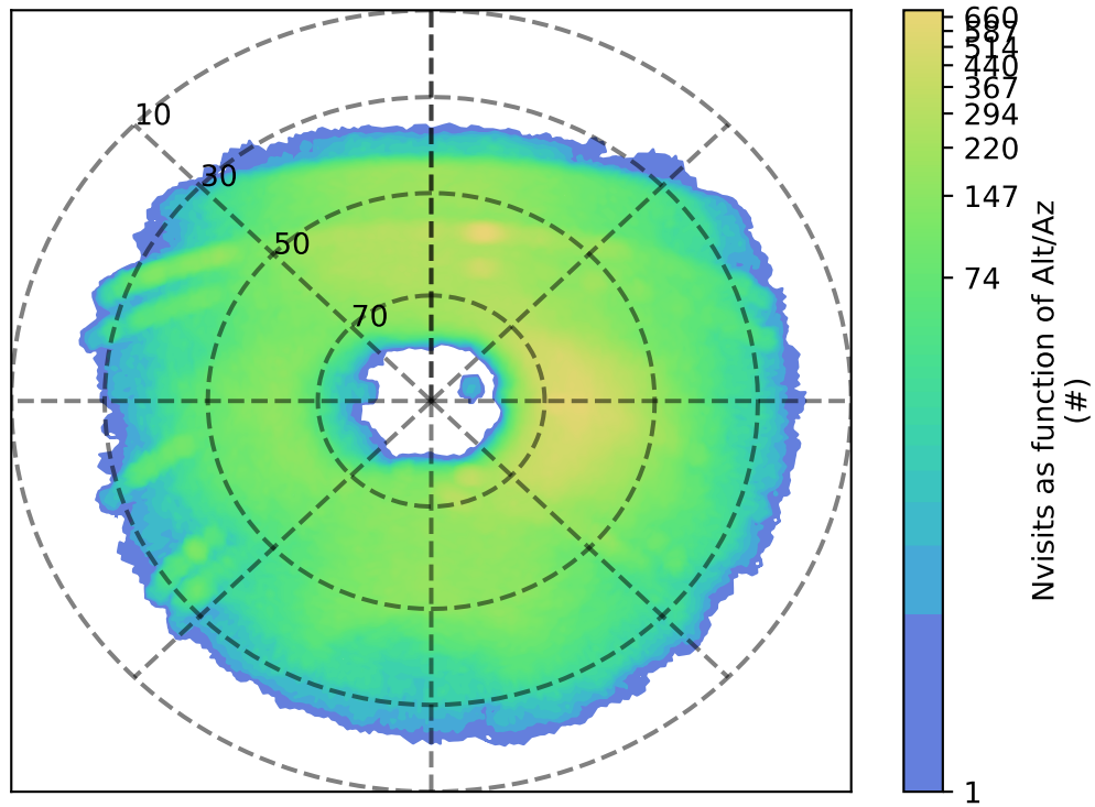
too_combined_s1.5_v3.4_10yrs u: Nvisits as function of Alt/Az
