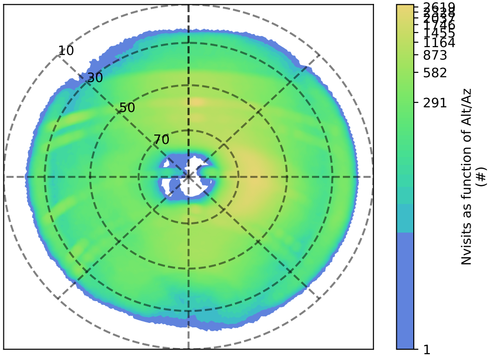
too_combined_s1.5_v3.4_10yrs i: Nvisits as function of Alt/Az
