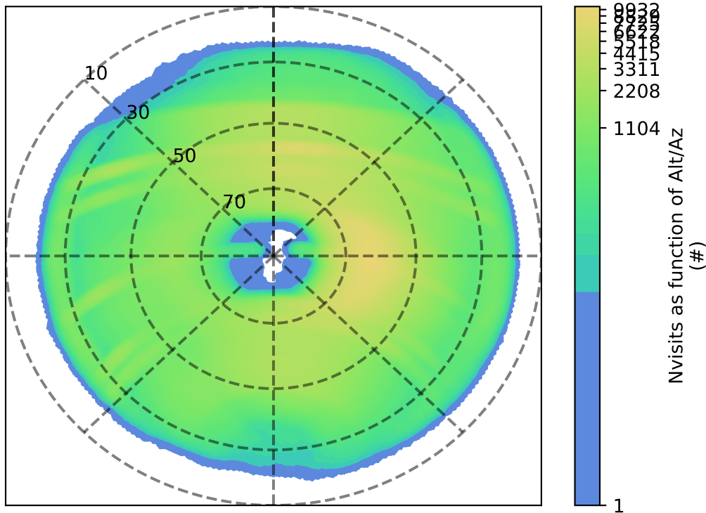
too_combined_s1.5_v3.4_10yrs : Nvisits as function of Alt/Az
