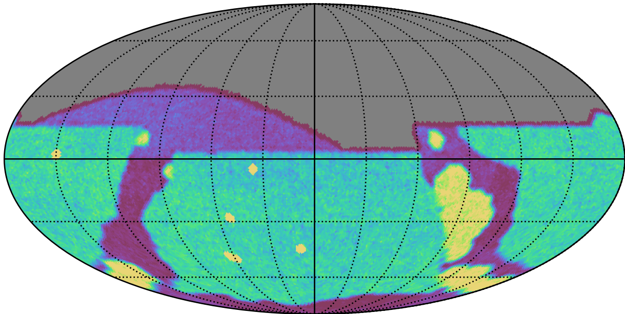
too_combined_s1.5_v3.4_10yrs g: Count observationStartMJD
