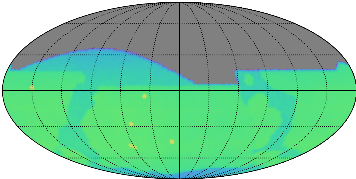
too_combined_s1.5_v3.4_10yrs r: CoaddM5
