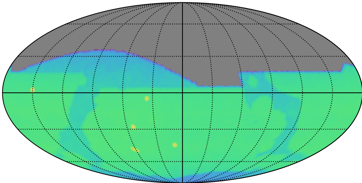
too_combined_s1.5_v3.4_10yrs i: CoaddM5
