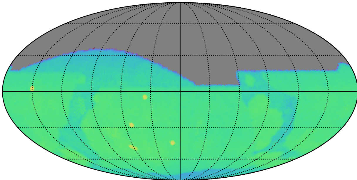
too_combined_s1.5_v3.4_10yrs g: CoaddM5
