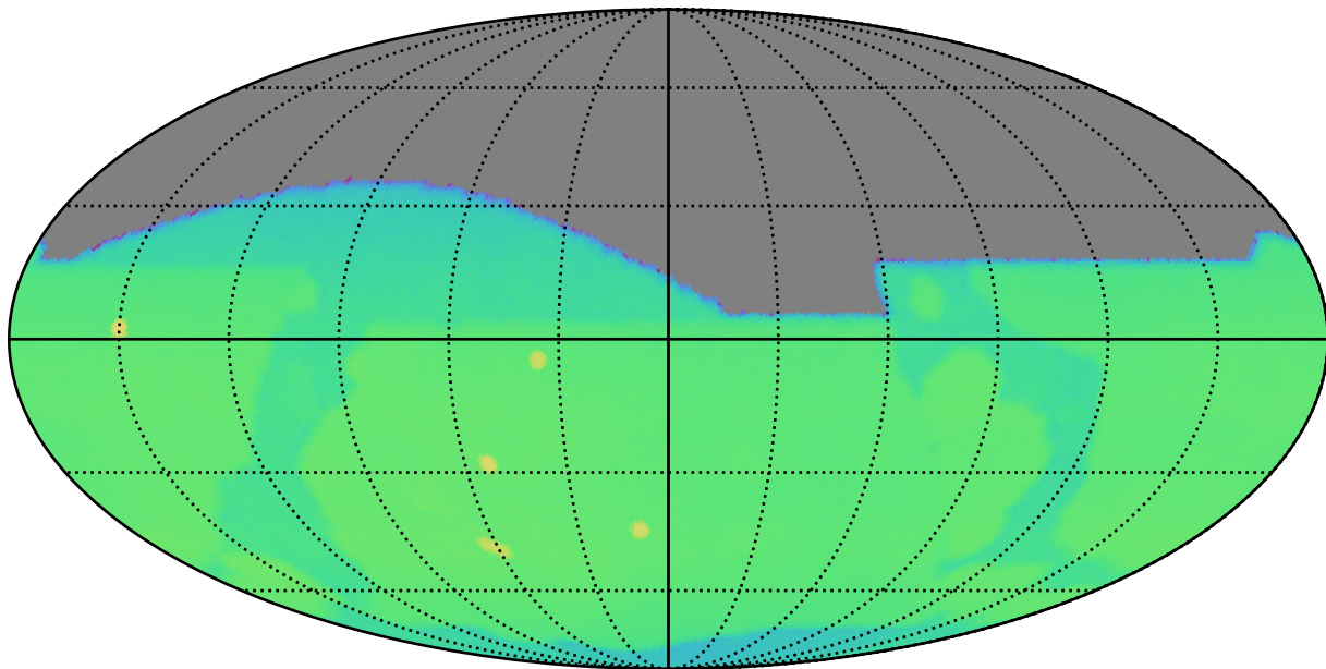
too_combined_s1.5_v3.4_10yrs : CoaddM5
