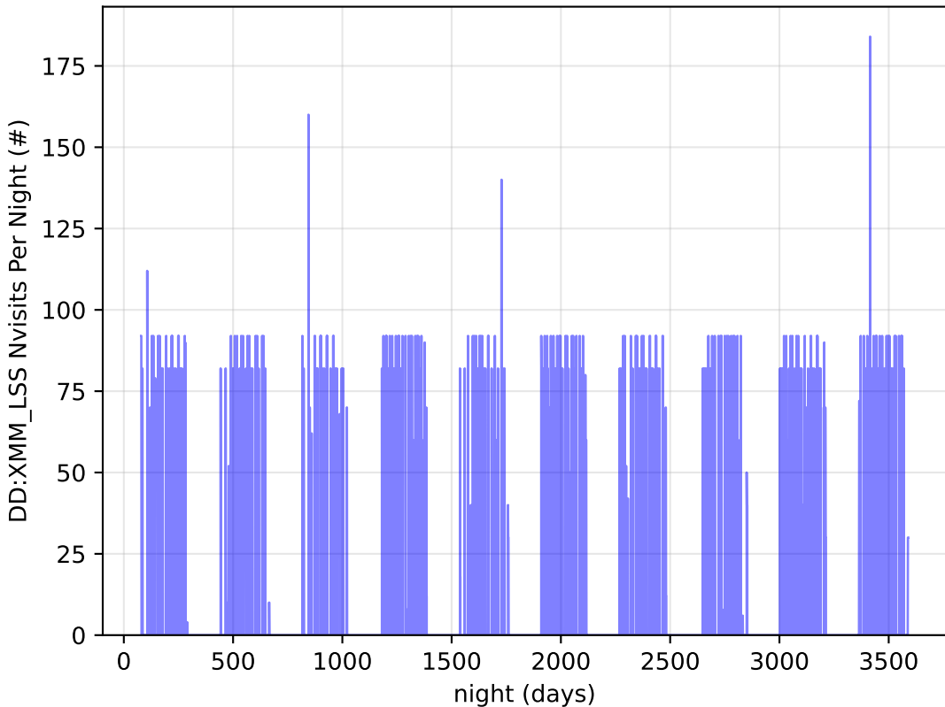
too_combined_s1.5_v3.4_10yrs all bands: DD:XMM_LSS Nvisits Per Night
