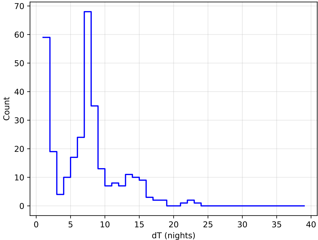
too_combined_s1.5_v3.4_10yrs all bands: DD:XMM_LSS Delta Nights Histogram
