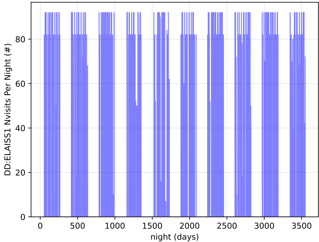
too_combined_s1.5_v3.4_10yrs all bands: DD:ELAISS1 Nvisits Per Night
