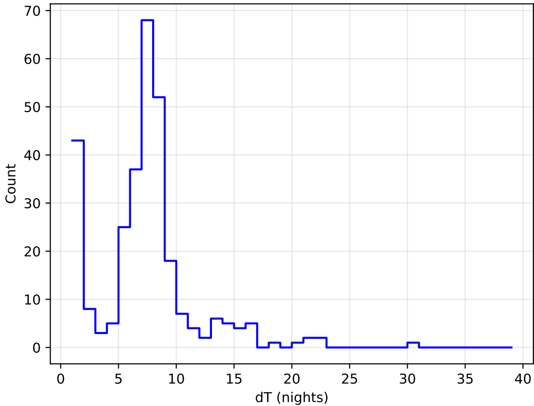
too_combined_s1.5_v3.4_10yrs all bands: DD:ELAISS1 Delta Nights Histogram
