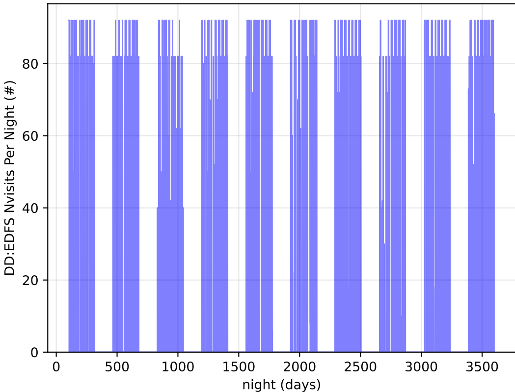
too_combined_s1.5_v3.4_10yrs all bands: DD:EDFS Nvisits Per Night
