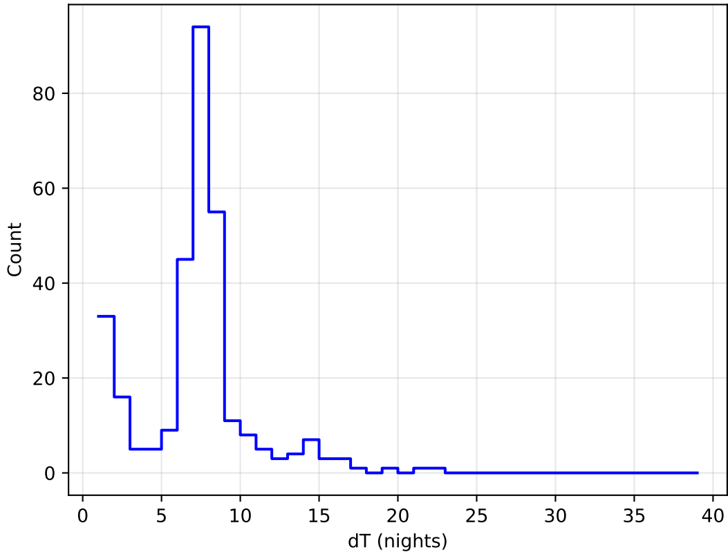
too_combined_s1.5_v3.4_10yrs all bands: DD:EDFS Delta Nights Histogram
