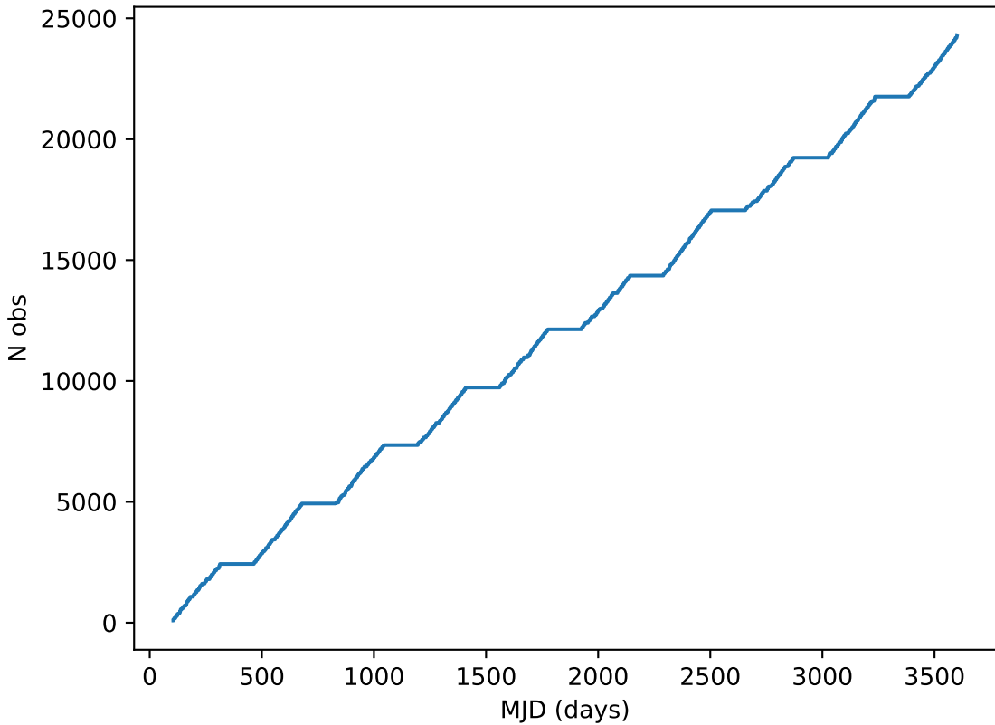
too_combined_s1.5_v3.4_10yrs all bands: DD:EDFS Cumulative NVisits
