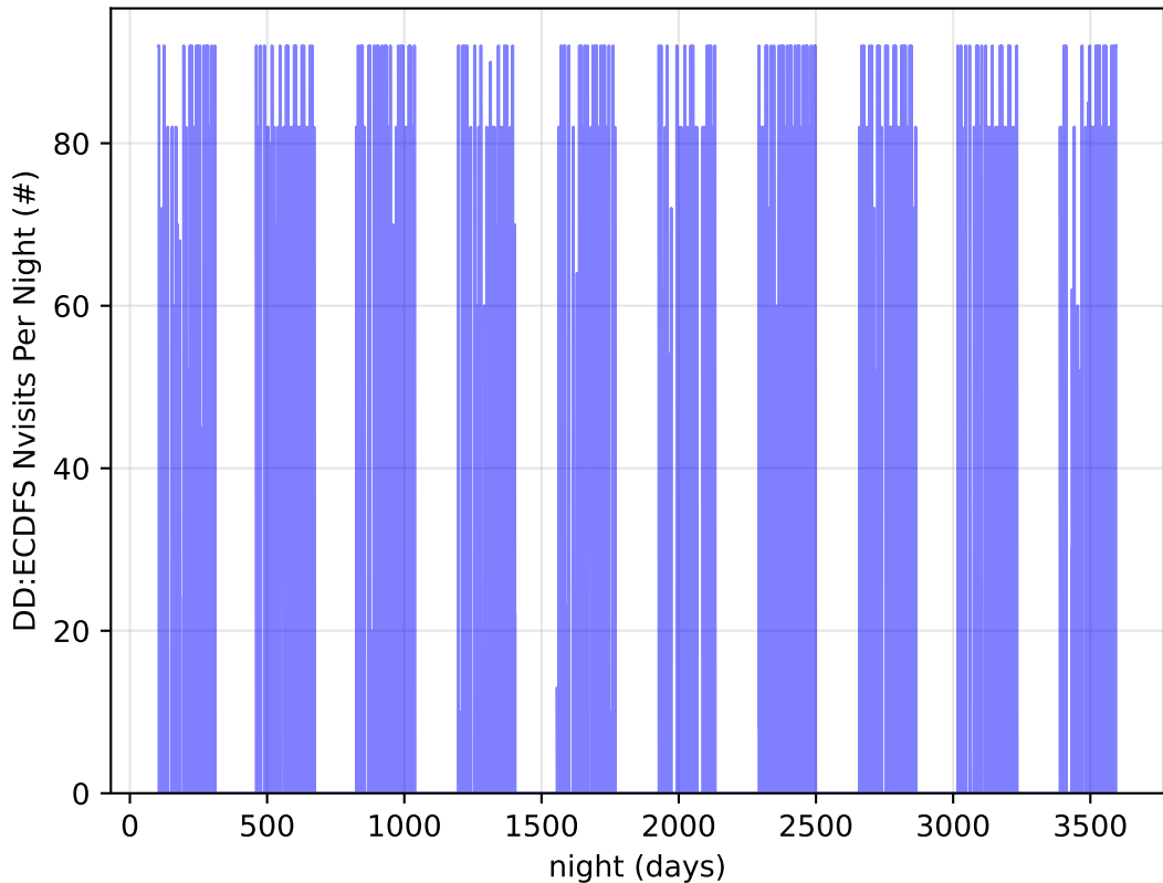
too_combined_s1.5_v3.4_10yrs all bands: DD:ECDFS Nvisits Per Night
