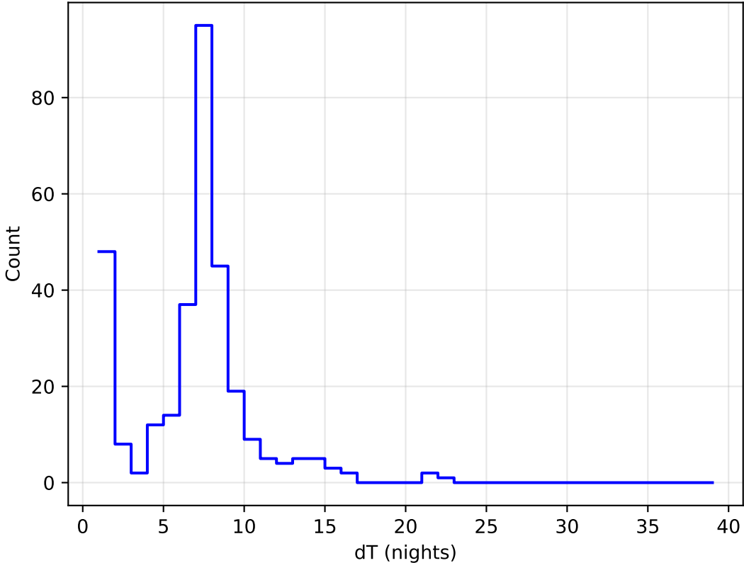
too_combined_s1.5_v3.4_10yrs all bands: DD:ECDFS Delta Nights Histogram
