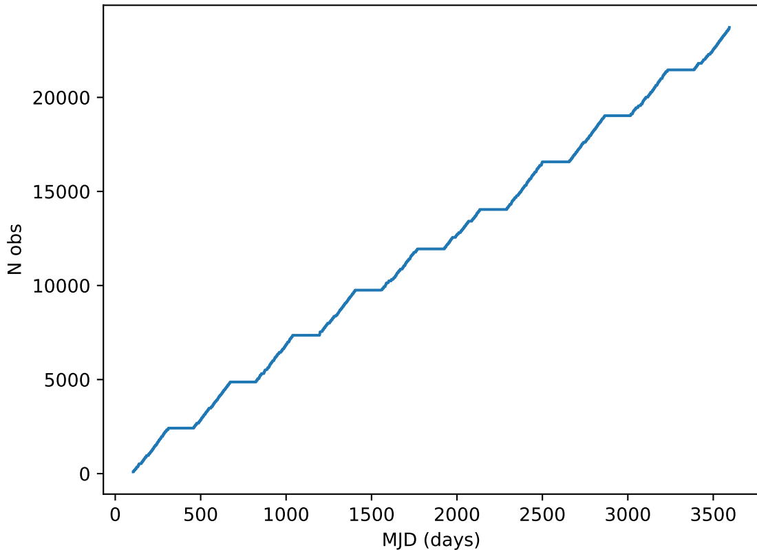
too_combined_s1.5_v3.4_10yrs all bands: DD:ECDFS Cumulative NVisits
