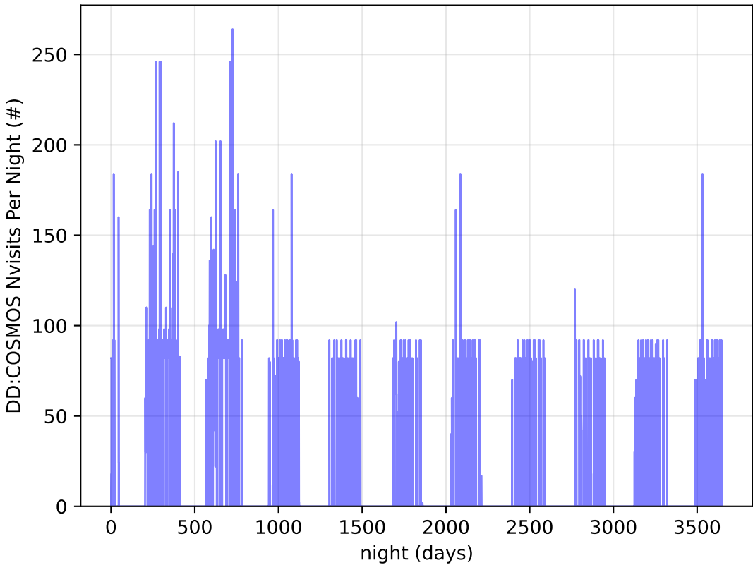
too_combined_s1.5_v3.4_10yrs all bands: DD:COSMOS Nvisits Per Night
