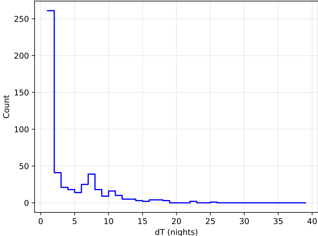
too_combined_s1.5_v3.4_10yrs all bands: DD: COSMOS Delta Nights Histogram
