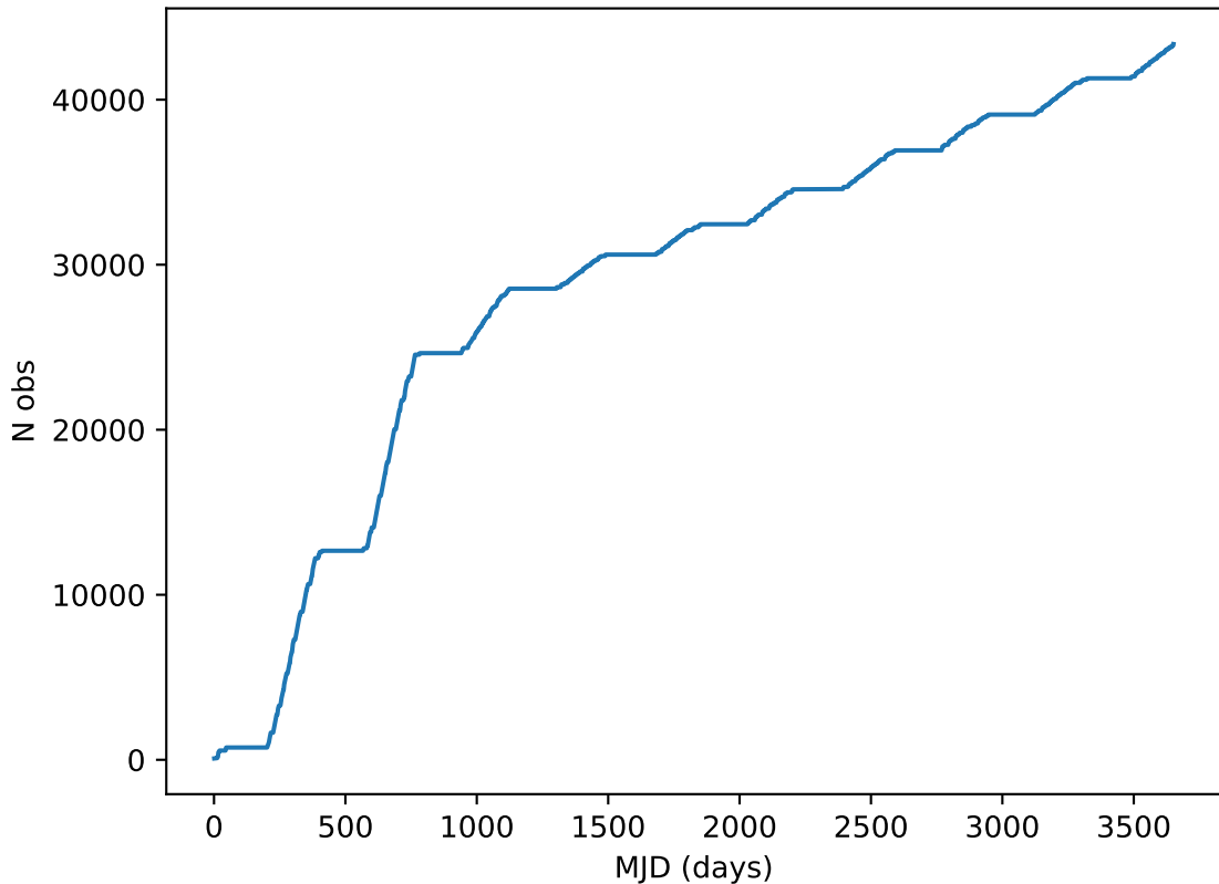
too_combined_s1.5_v3.4_10yrs all bands: DD: COSMOS Cumulative NVisits
