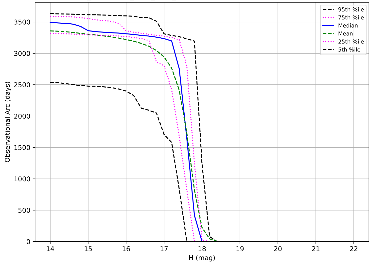
too_combined_s1.0_v3.4_10yrs: Observational Arc Length Trojan
