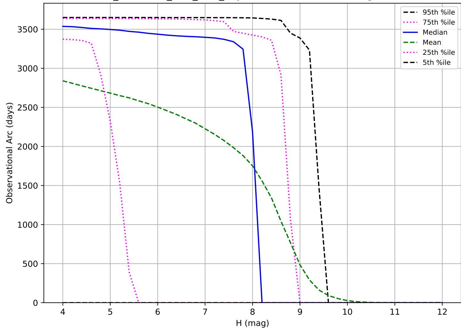
too_combined_s1.0_v3.4_10yrs: Observational Arc Length TNO
