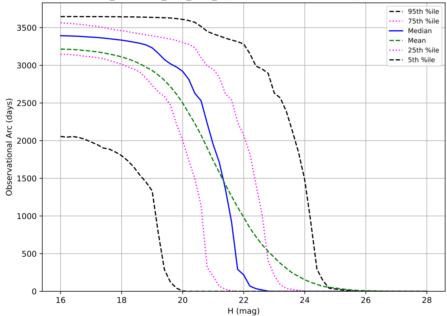
too_combined_s1.0_v3.4_10yrs: Observational Arc Length PHA
