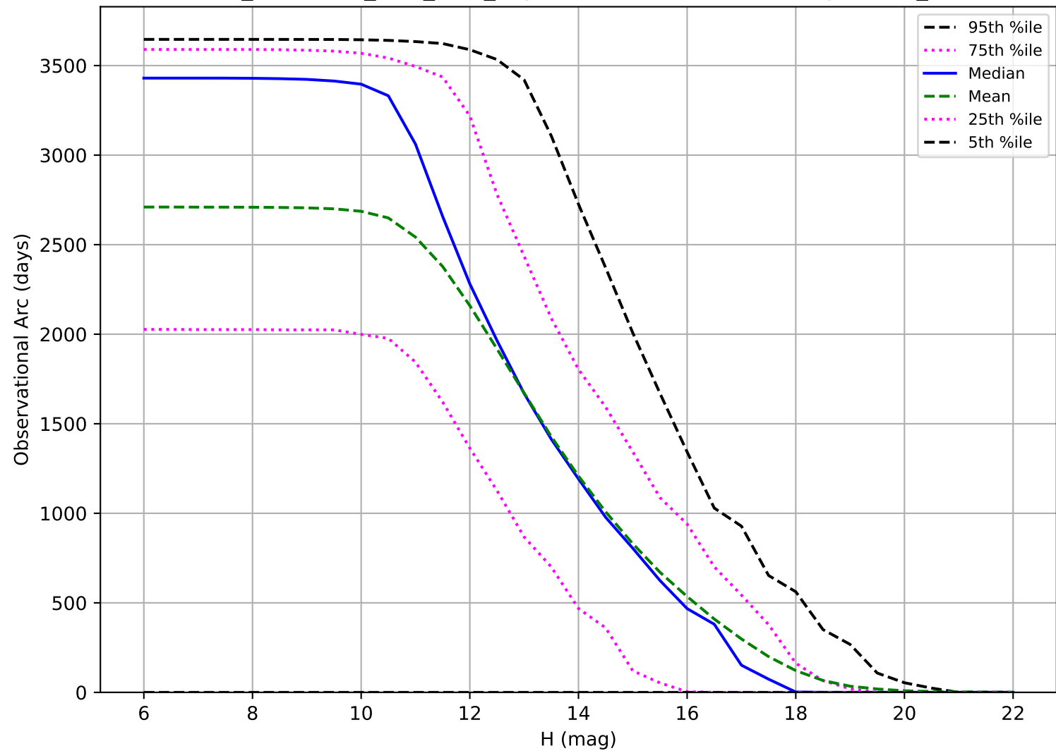
too_combined_s1.0_v3.4_10yrs: Observational Arc Length OCC_r5
