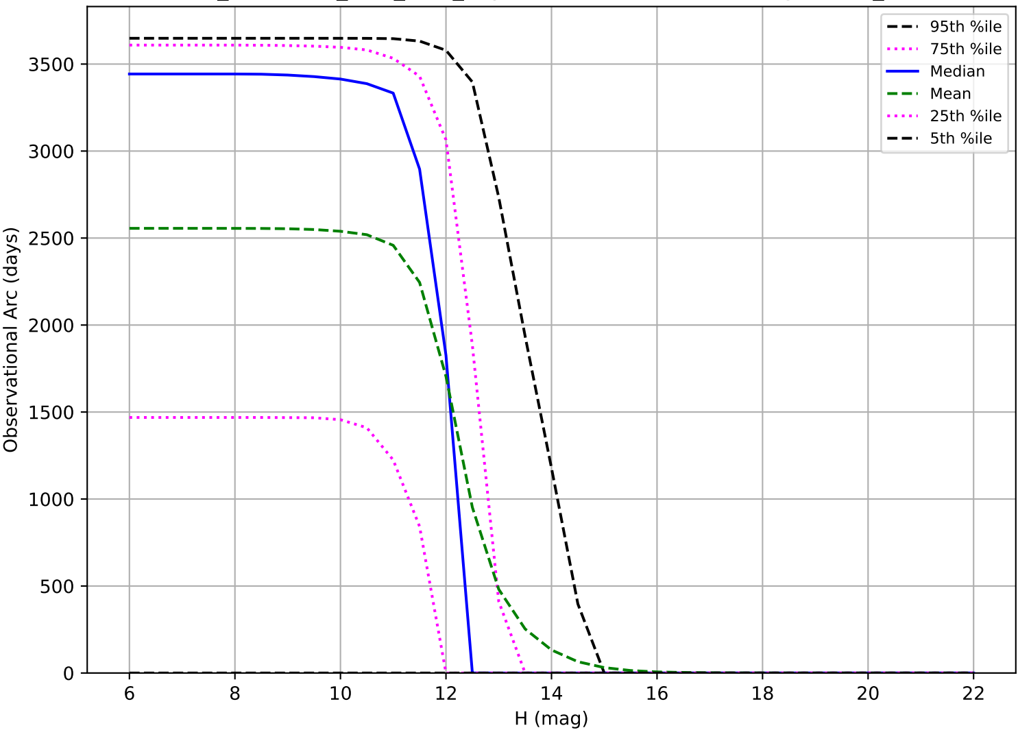
too_combined_s1.0_v3.4_10yrs: Observational Arc Length OCC_r20
