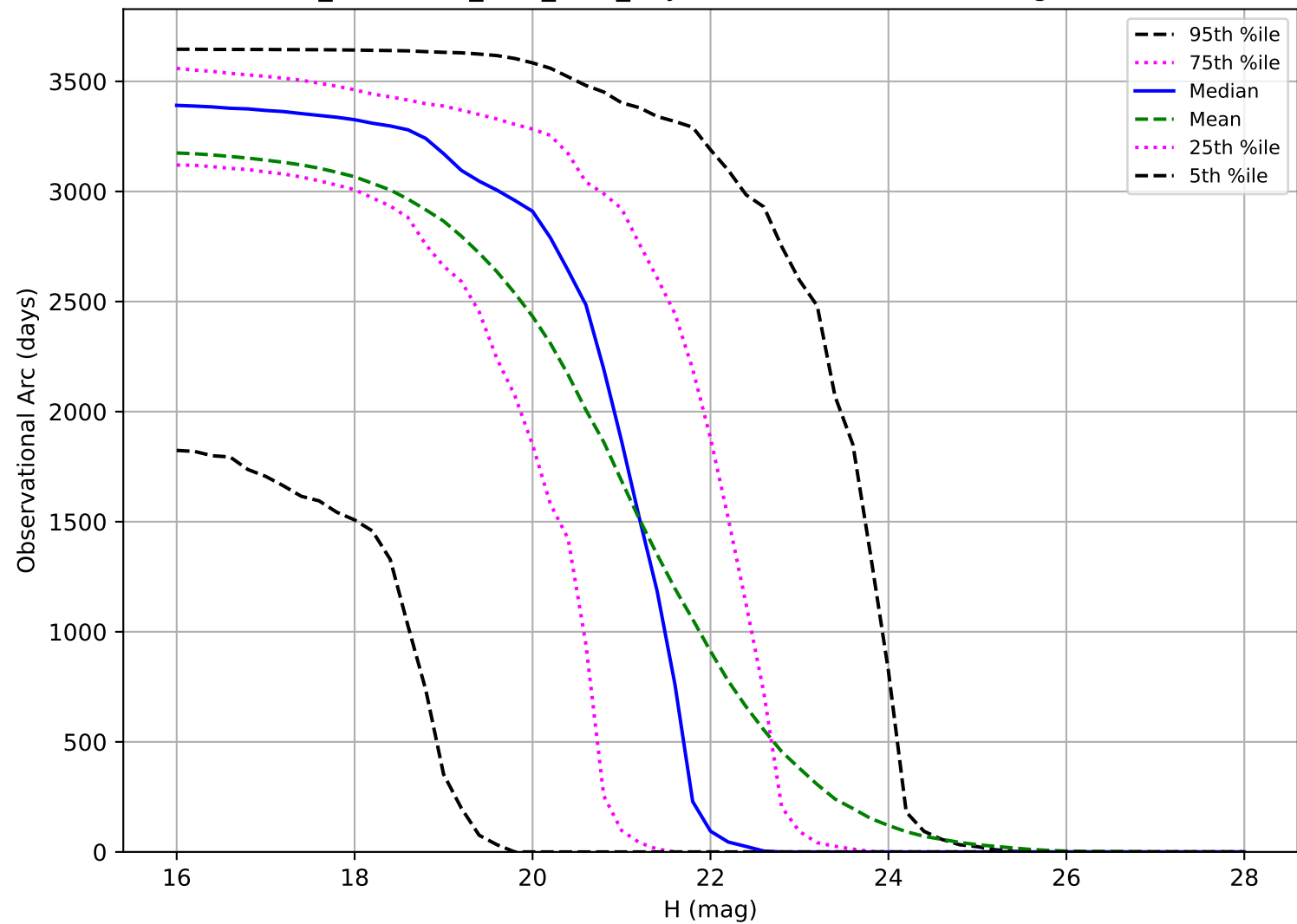
too_combined_s1.0_v3.4_10yrs: Observational Arc Length NEO
