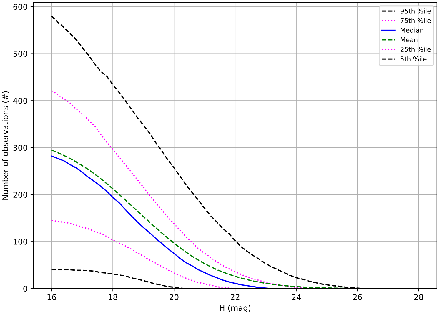
too_combined_s1.0_v3.4_10yrs: Number of observations PHA
