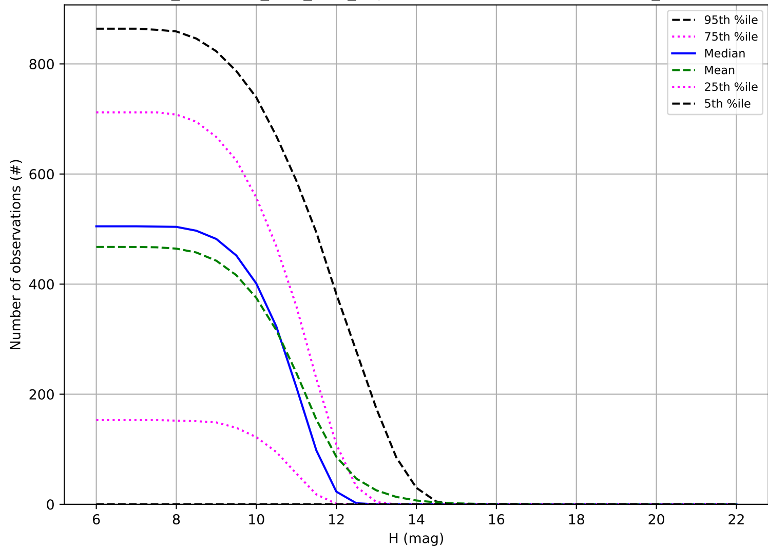
too_combined_s1.0_v3.4_10yrs: Number of observations OCC_r20
