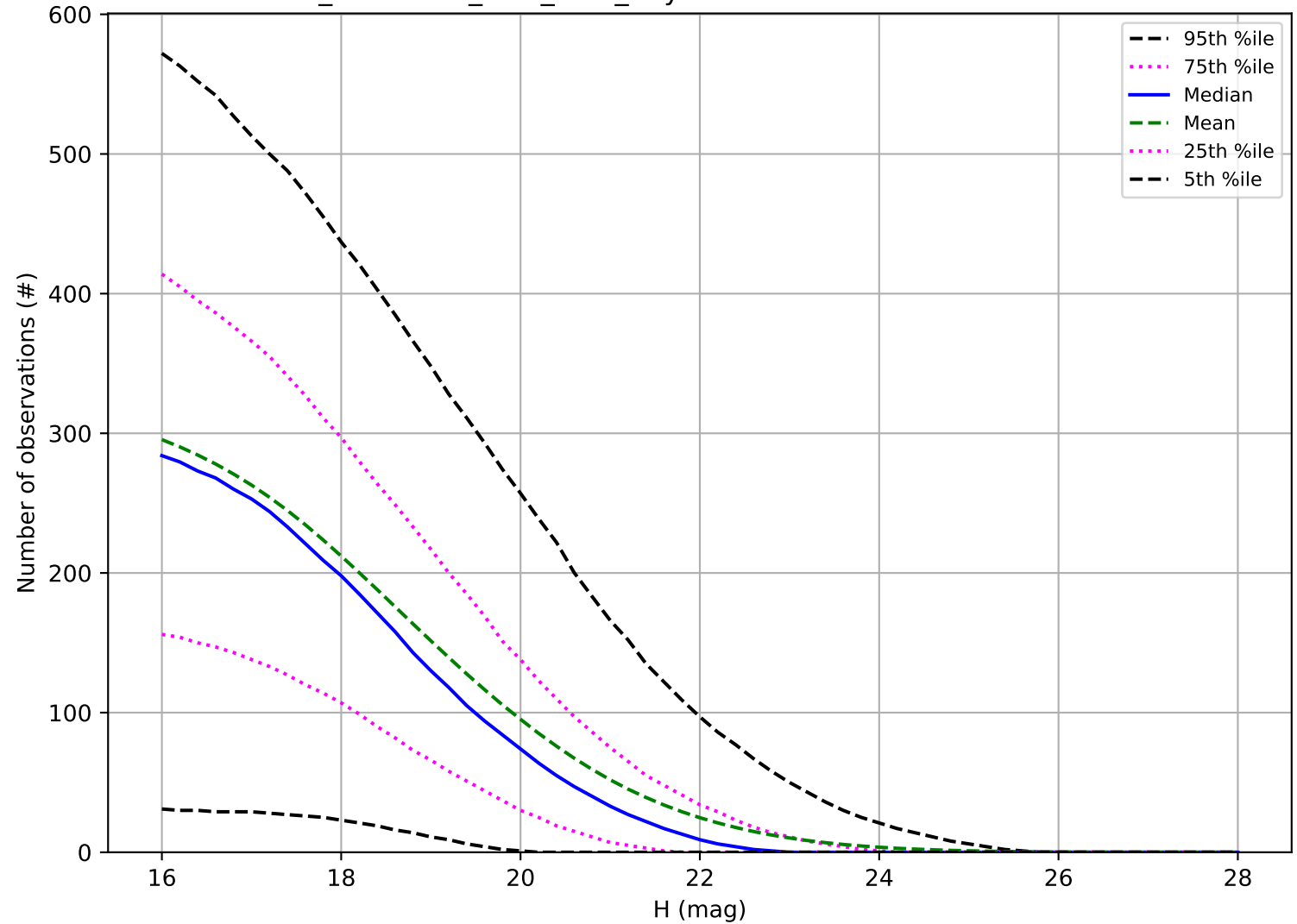
too_combined_s1.0_v3.4_10yrs: Number of observations NEO
