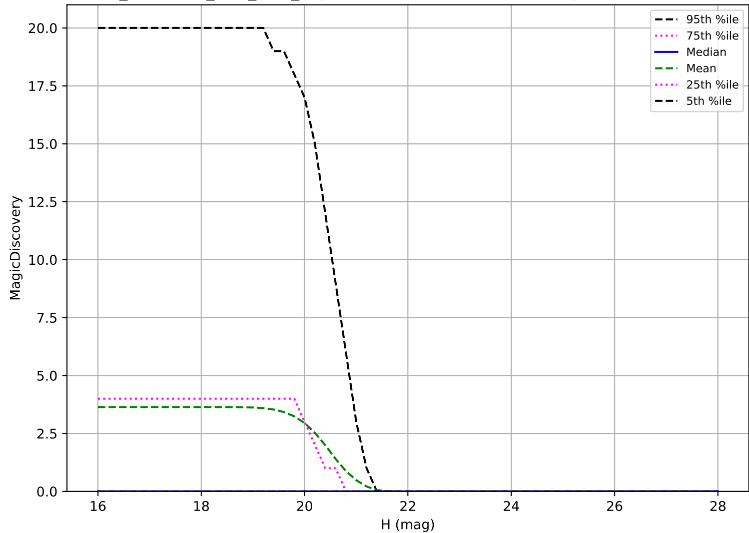
too_combined_s1.0_v3.4_10yrs: Vatira 6 detections in 60 nights detection loss
