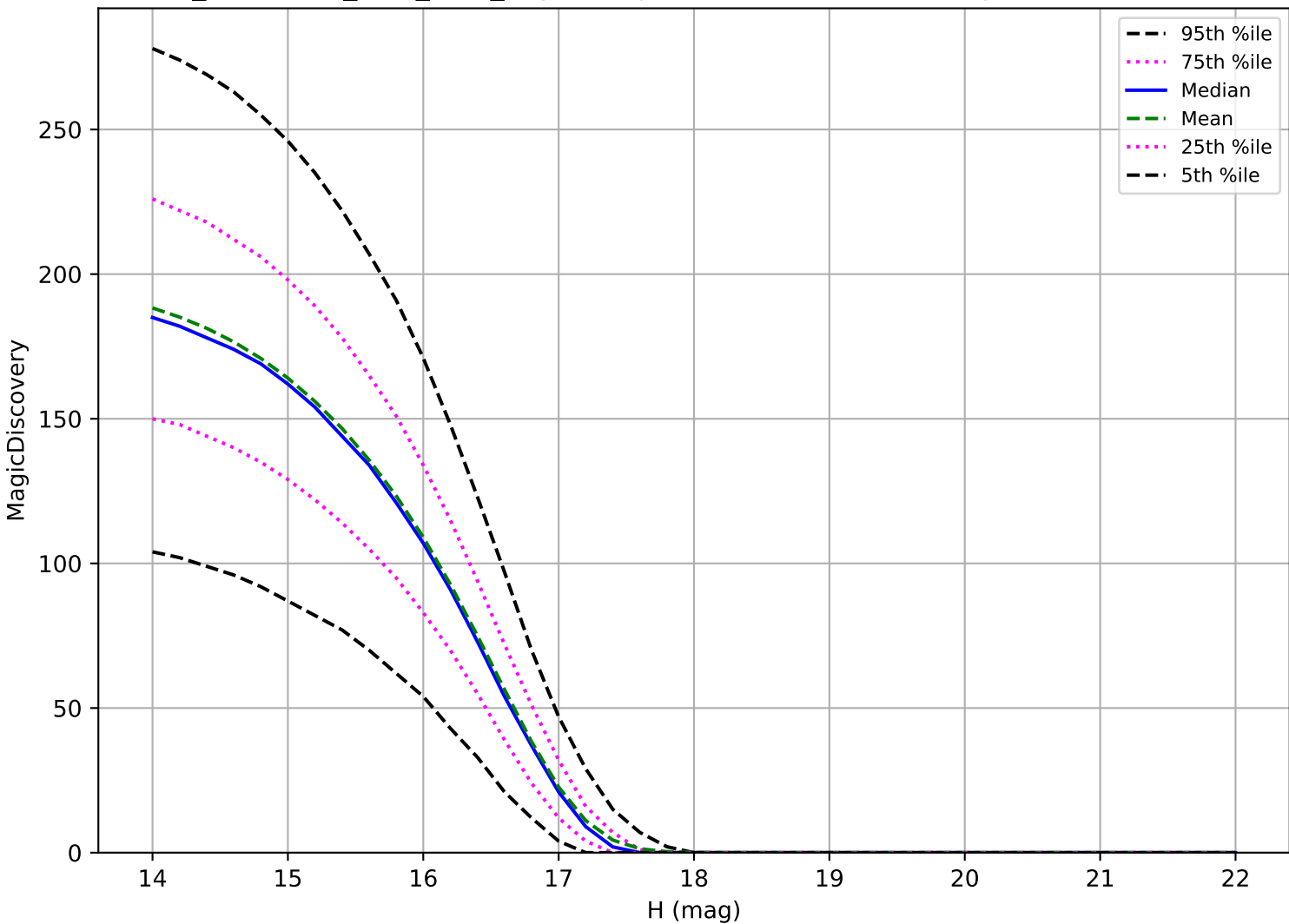
too_combined_s1.0_v3.4_10yrs: Trojan 6 detections in 60 nights detection loss
