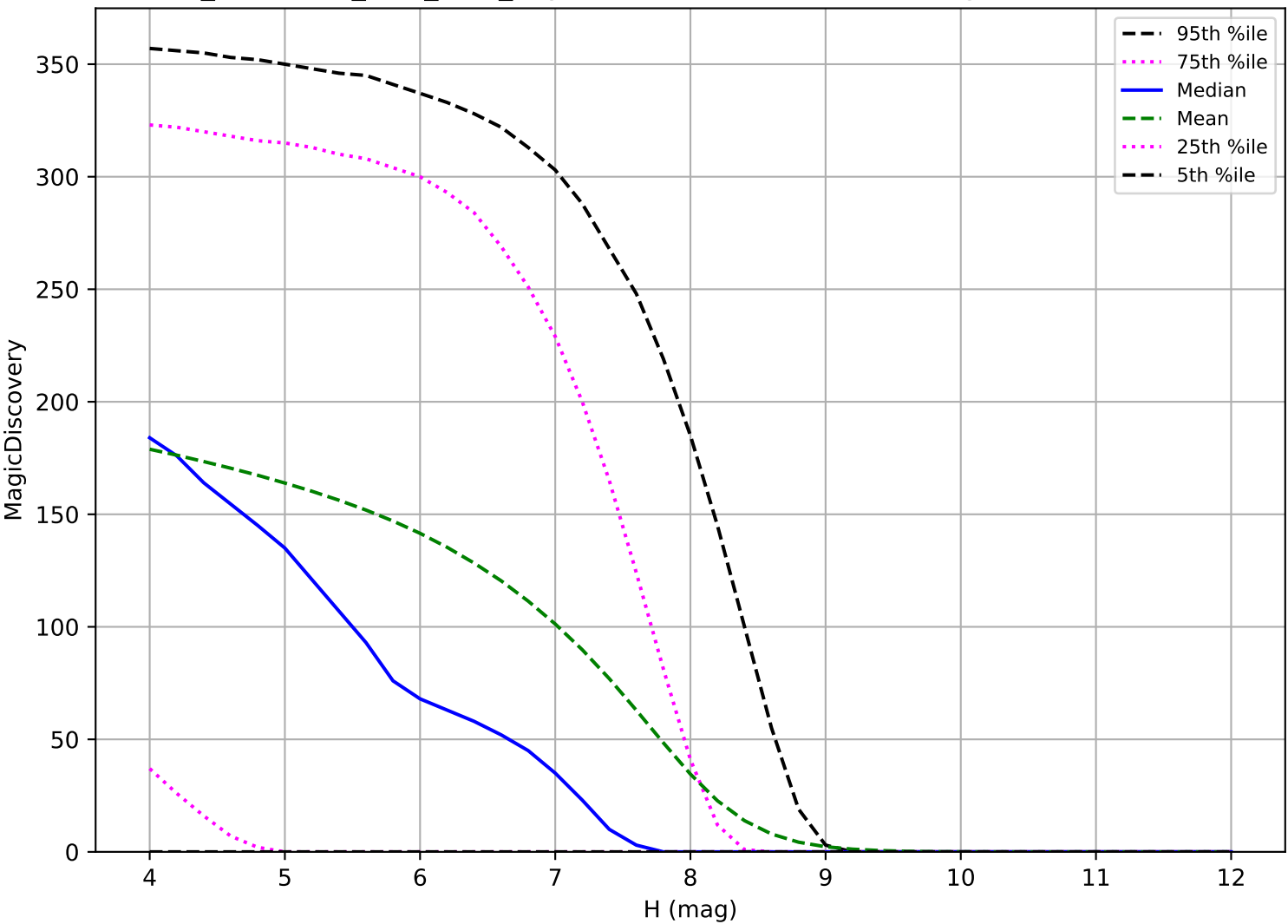
too_combined_s1.0_v3.4_10yrs: TNO 6 detections in 60 nights detection loss
