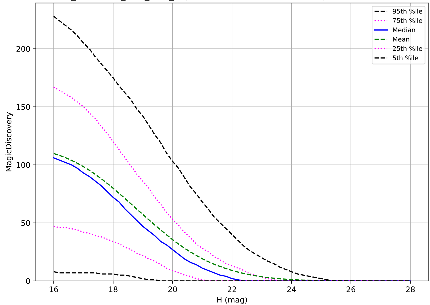
too_combined_s1.0_v3.4_10yrs: PHA 6 detections in 60 nights detection loss
